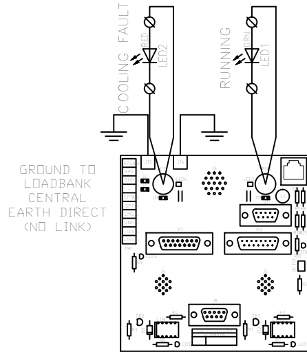
COMMS. BOARD PCB CL15851A
