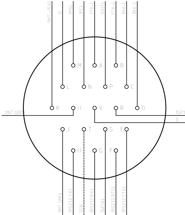
19-WAY MIL SOCKET IDENTIFICATION ON LOADBANK FACIA
